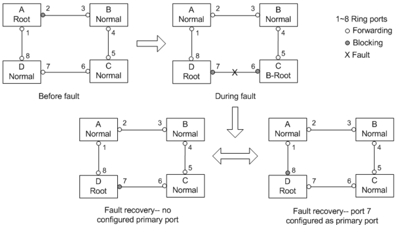
Figure 197 DRP Link Fault
