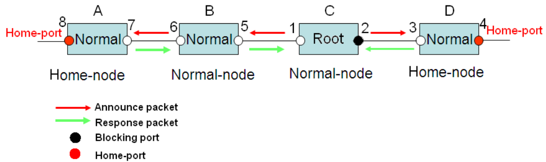
Figure 201 DHP Configuration
