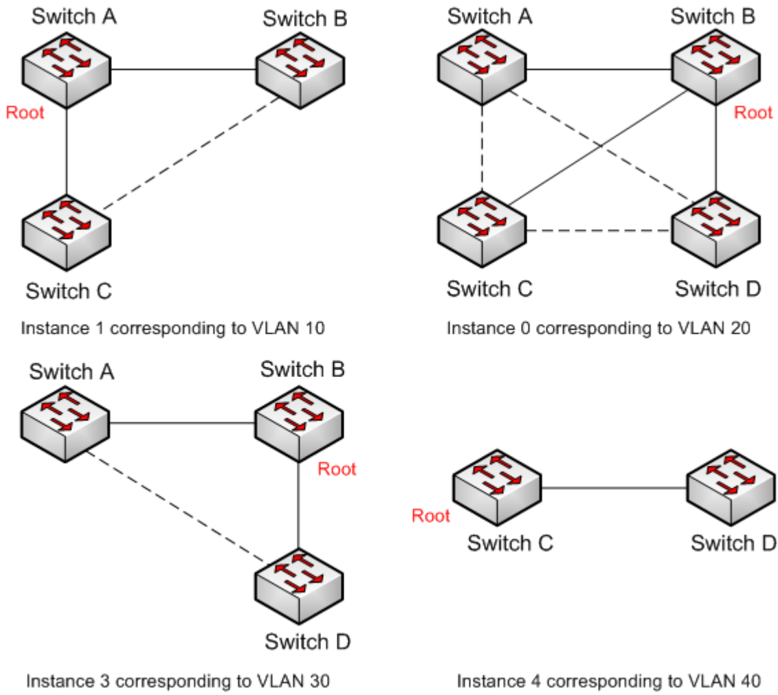
Figure 227 Spanning Tree Instance of each VLAN
