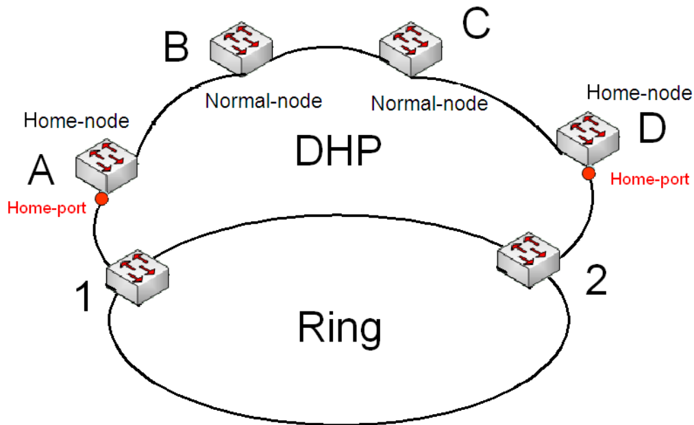
Figure 200 DHP Application
