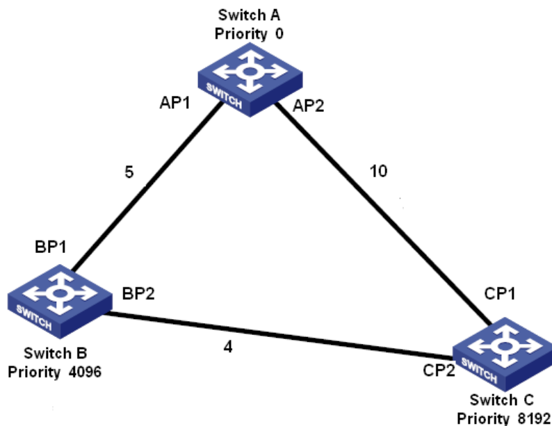
Figure 210 RSTP Configuration Example
