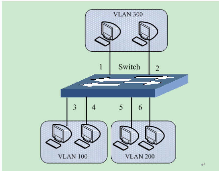
Figure 182 PVLAN Configuration Example
