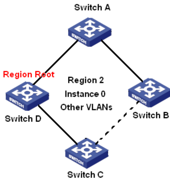
Figure 216 Other VLAN Mapping to Instance 0
