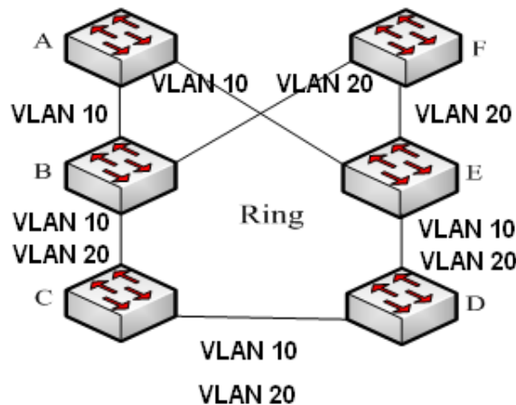
Figure 190 DT-Ring-VLAN
