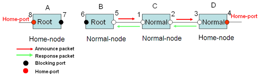
Figure 202 DHP Fault Recovery
