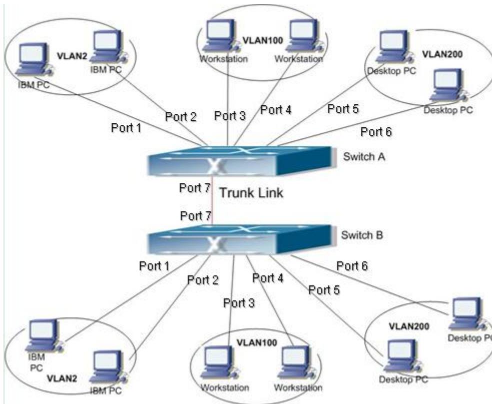
Figure 180 VLAN Application
