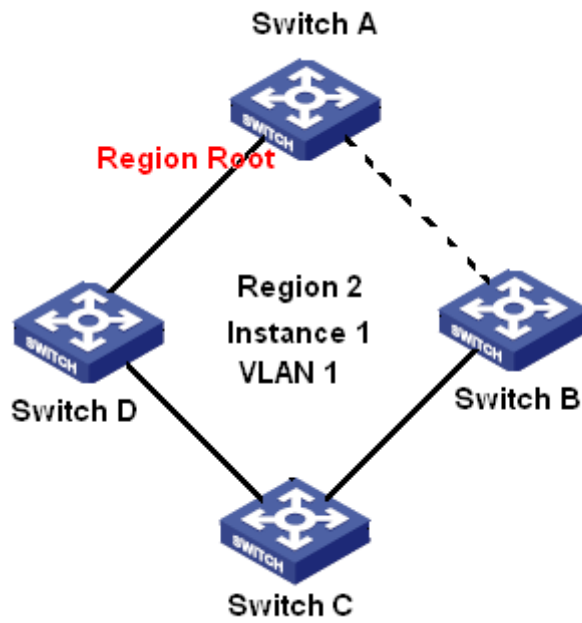
Figure 214 VLAN 1 Mapping to Instance 1
