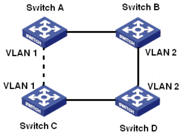
Figure 211 RSTP Disadvantage
