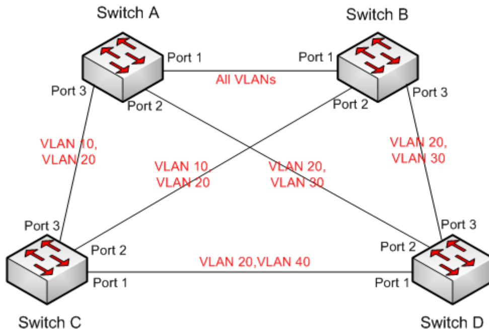
Figure 226 MSTP Typical Configuration Example
