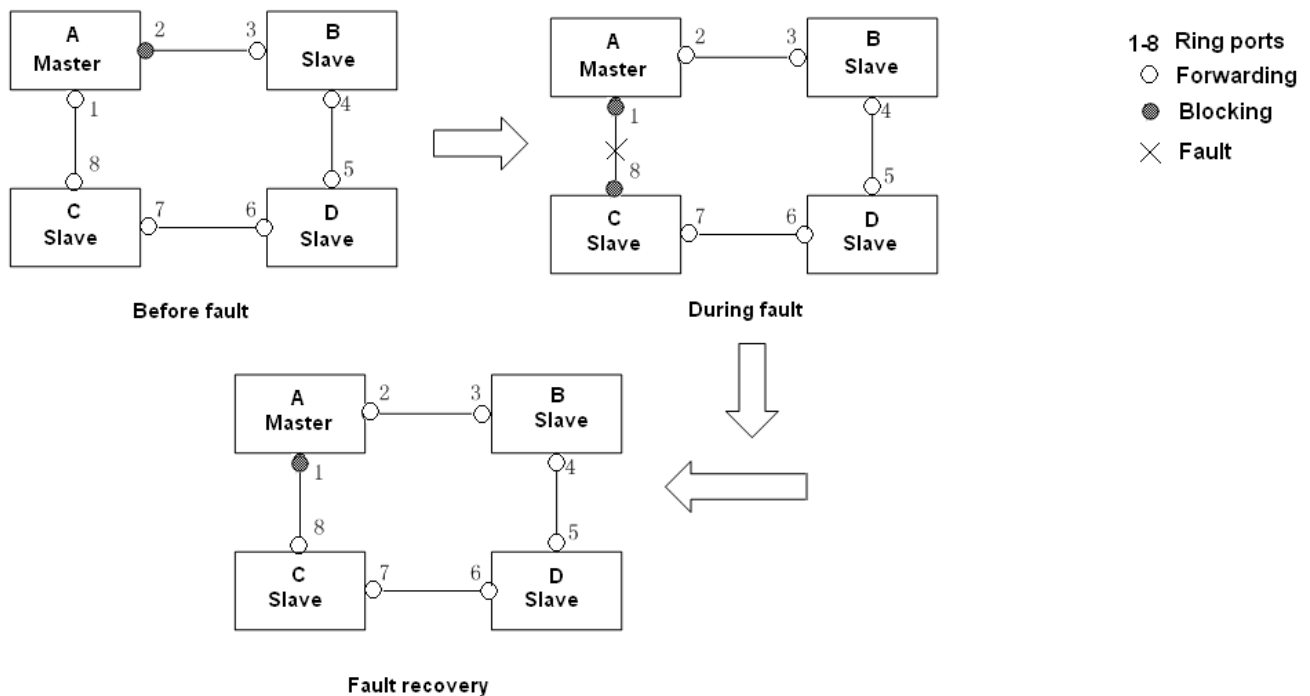
Figure 189 DT-Ring Link Fault
