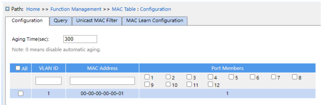
Figure 165 MAC Address Aging Time Configuration
