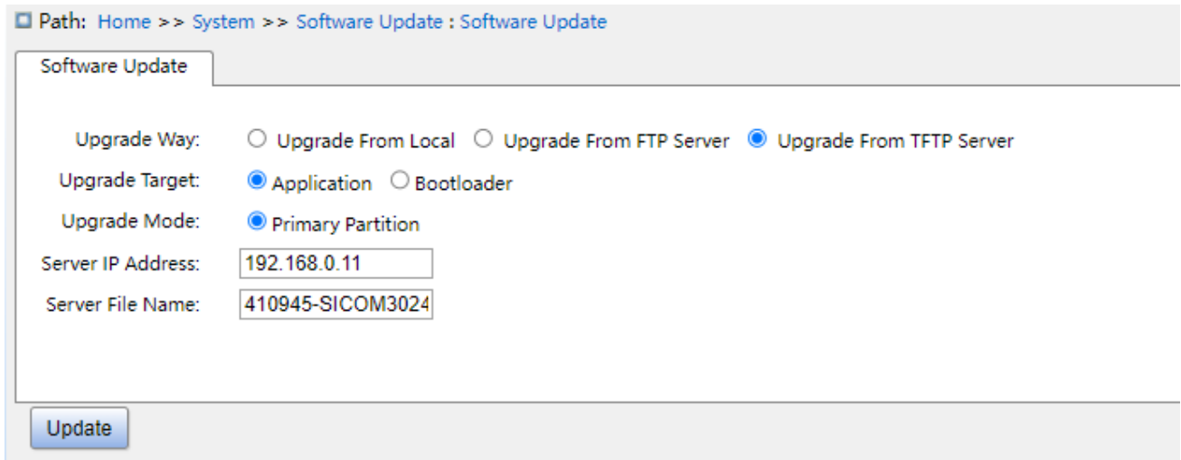
Figure 36 Software Update by TFTP
