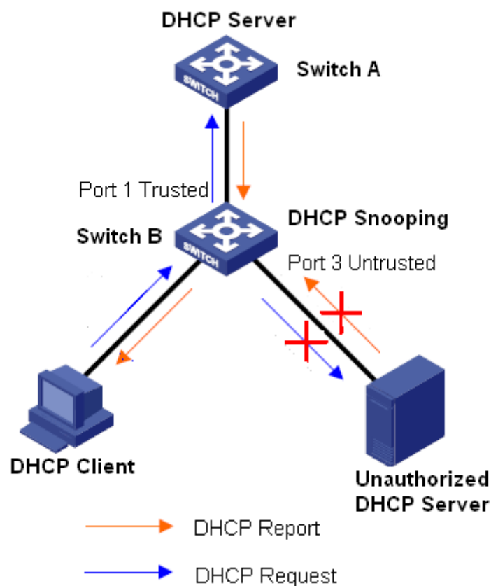
Figure 193 DHCP Snooping Typical Configuration Example
