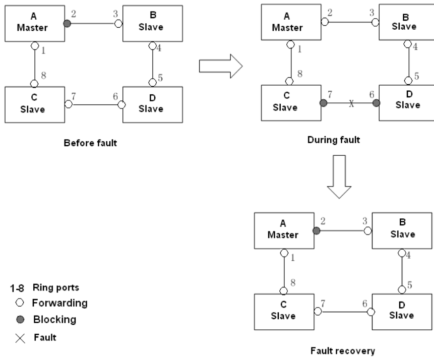
Figure 116 CD Link Fault
