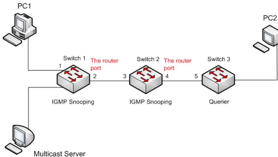
Figure 178 IGMP Snooping Application Example
