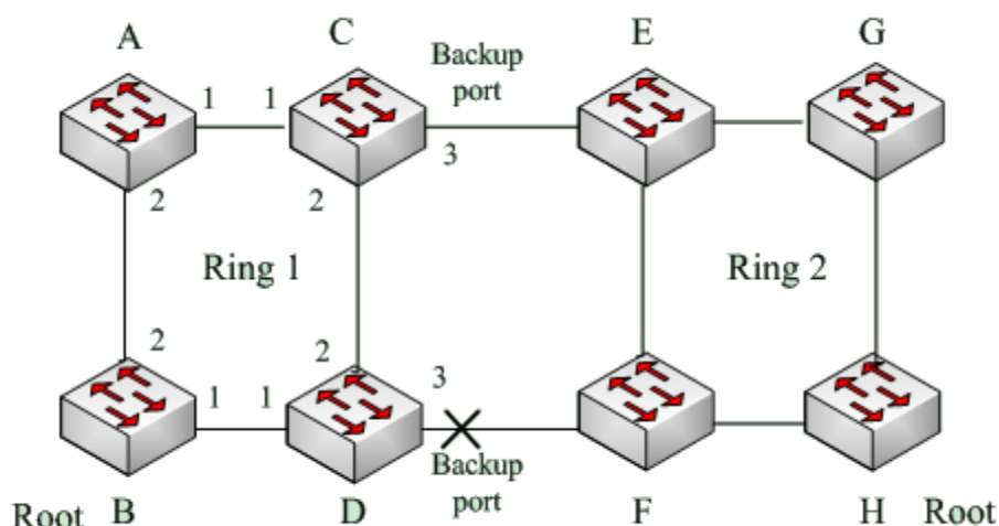
Figure 127 DRP Backup
