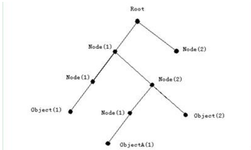
Figure 44 MIB Structure
