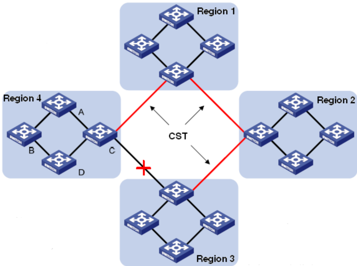
Figure 142 MSTP Concepts
