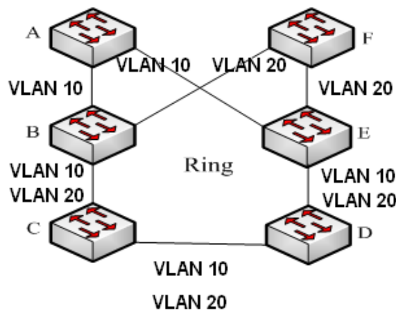
Figure 118 DT-Ring-VLAN
