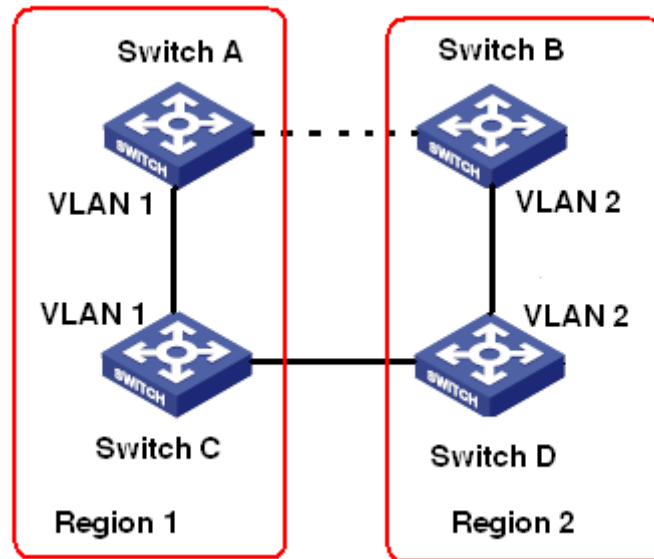
Figure 141 MSTP Topology
