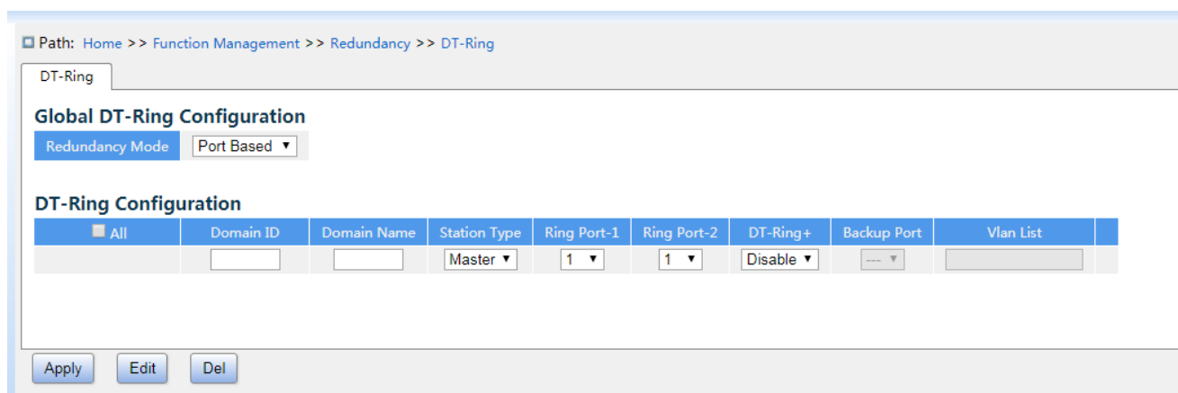
Figure 121 DT-Ring-Port Configuration
