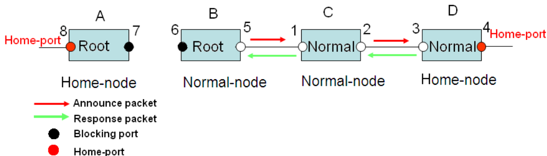
Figure 130 DHP Fault Recovery
