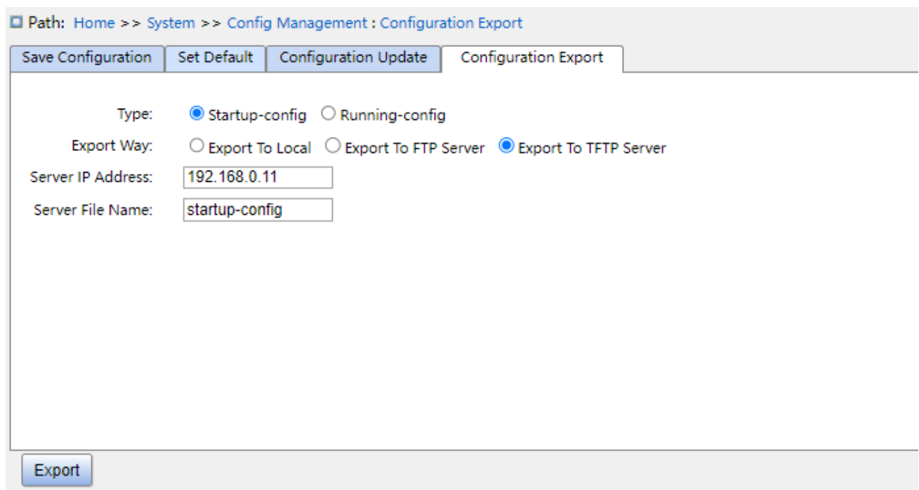
Figure 19 Export Configuration File-TFTP
