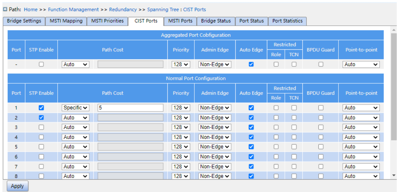
Figure 138 Configure RSTP Port
