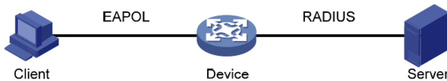
Figure 198 IEEE802.1X Structure
