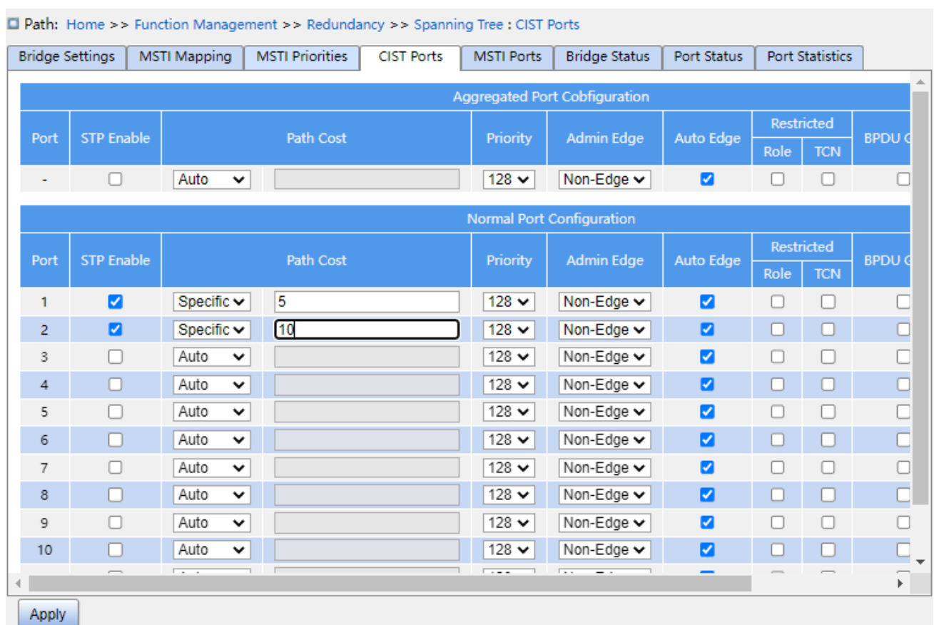
Figure 149 Configure CIST Ports
