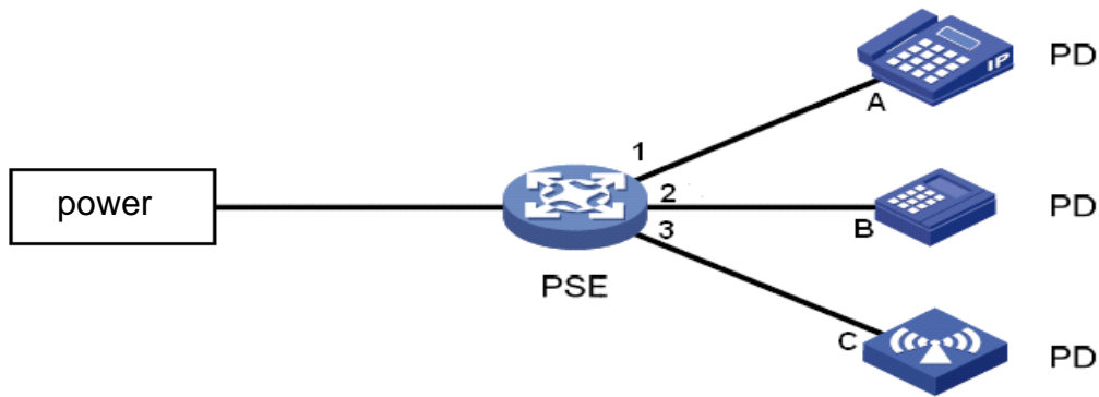
Figure 169 POE power supply system
