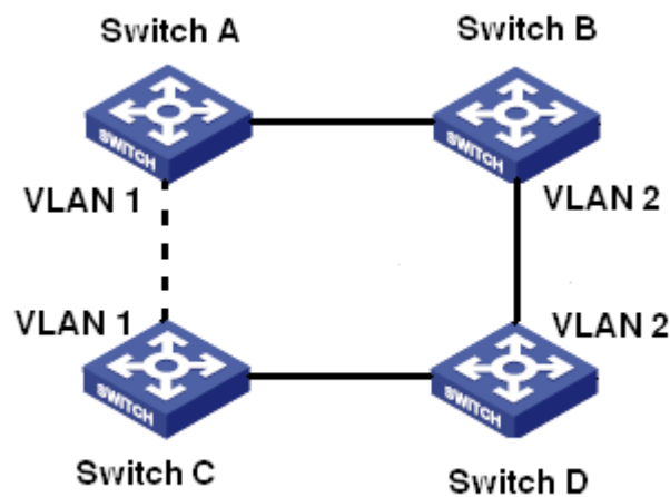
Figure 140 RSTP Disadvantage
