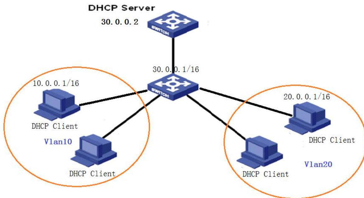
Figure 194 Client—Relay—Server Mode
