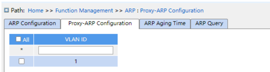
Figure 157 Proxy ARP Configuration
