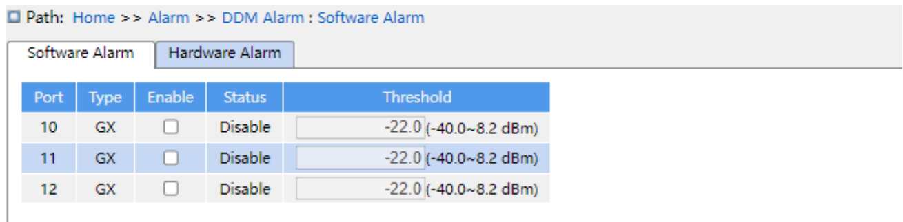
Figure 86 SFP port RX Power alarm
