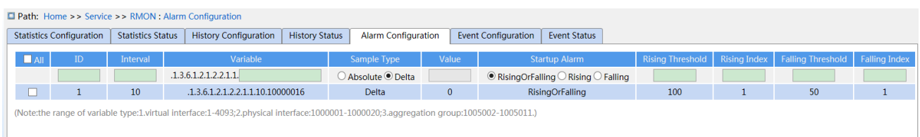
Figure 80 Configure Alarm Table
