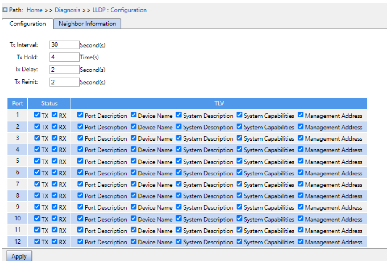
Figure 238 Configure LLDP
