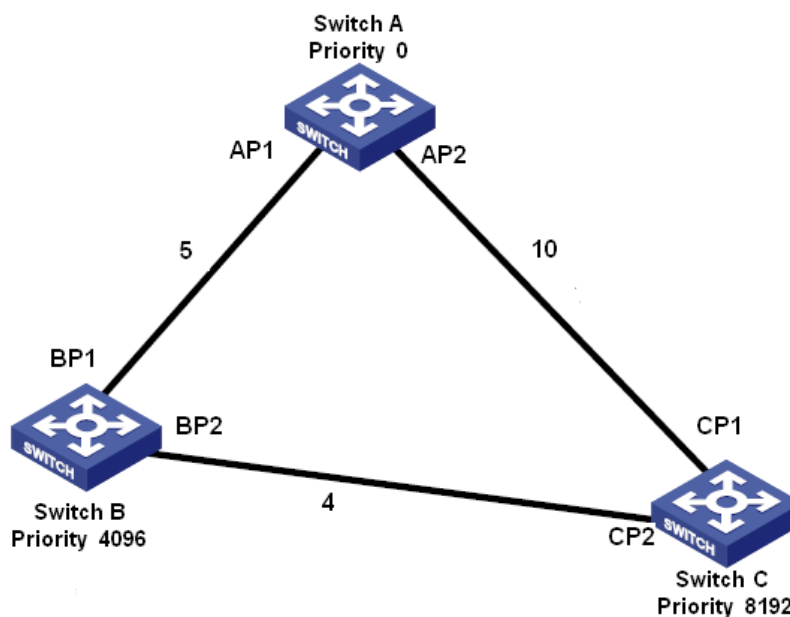
Figure 139 RSTP Configuration Example
