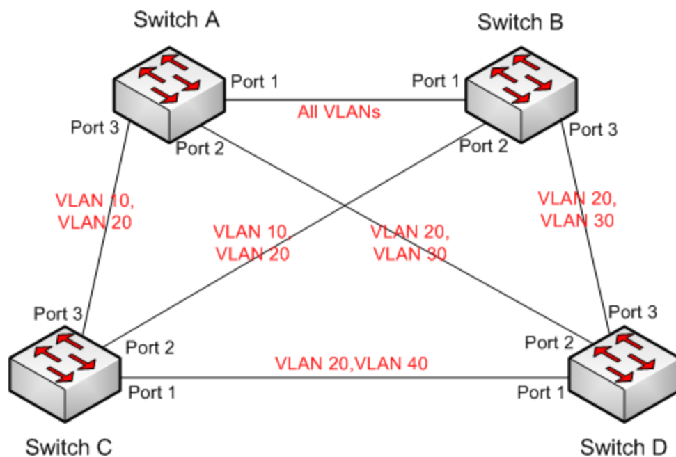
Figure 154 MSTP Typical Configuration Example
