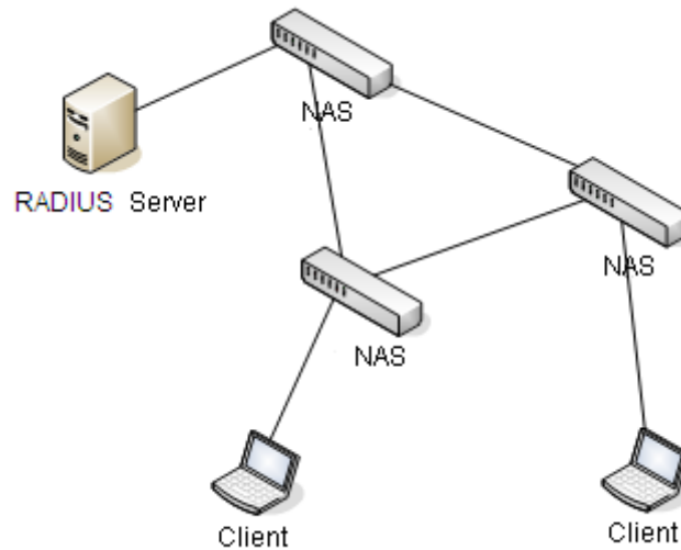
Figure 68 RADIUS Structure
