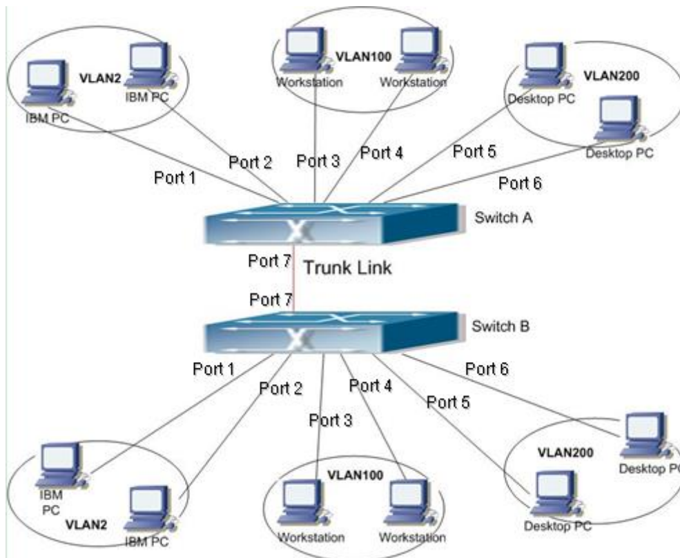
Figure 100 VLAN Application
