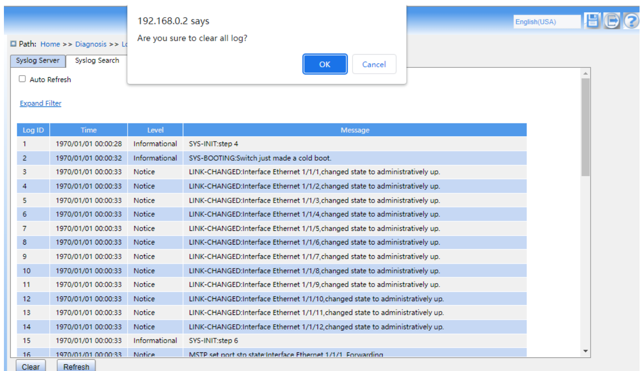
Figure 233 Clear logs
