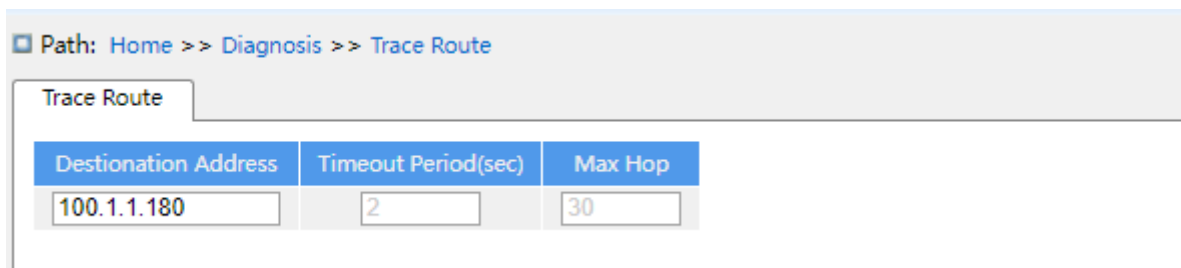
Figure 240 Configure Traceroute
