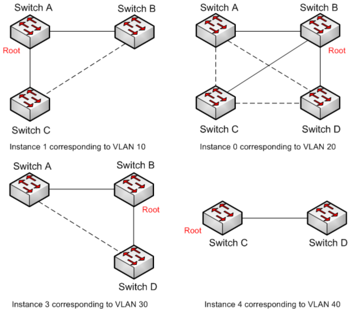
Figure 155 Spanning Tree Instance of each VLAN
