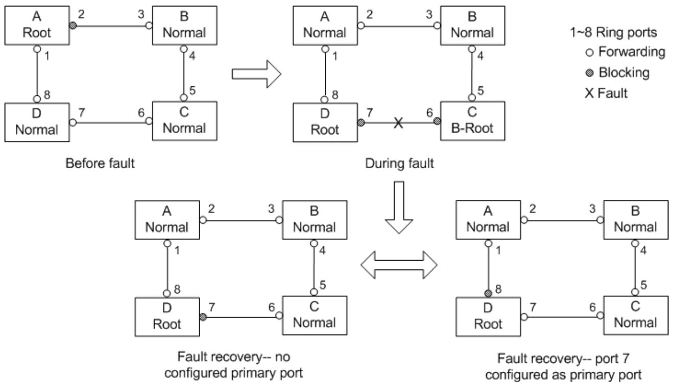
Figure 125 DRP Link Fault
