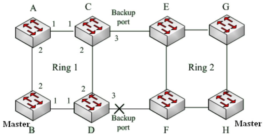
Figure 119 DT-Ring+ Topology
