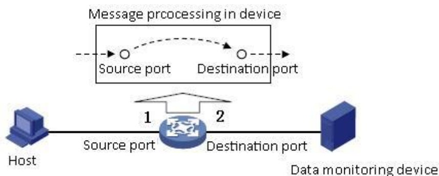
Figure 237 Port Mirror Example
